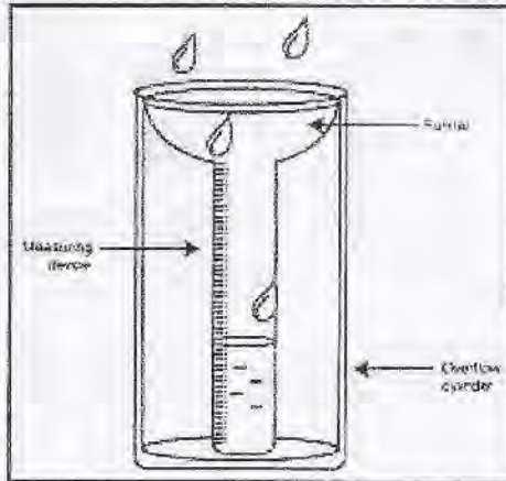
FIG. 151.—Standard rain-gauge.
